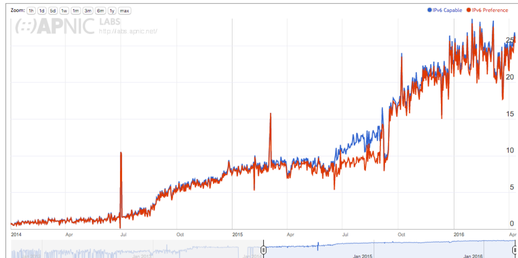
Use of IPv6 for Greece (GR)
