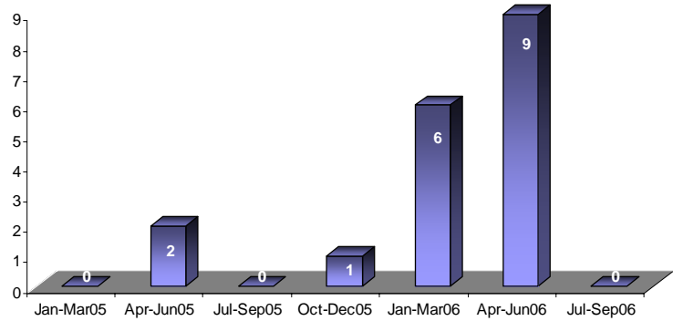
/32 IPv6 allocations
